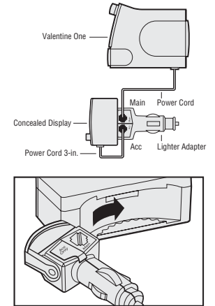
Lighter Adapter slides into place.
